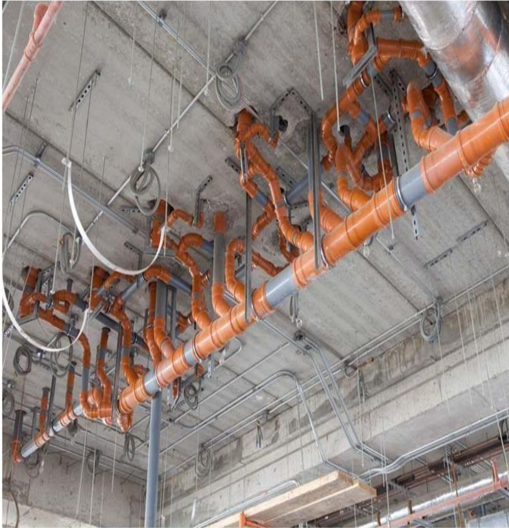
DRAINAGE SYSTEMS MECHANICAL WORKS
