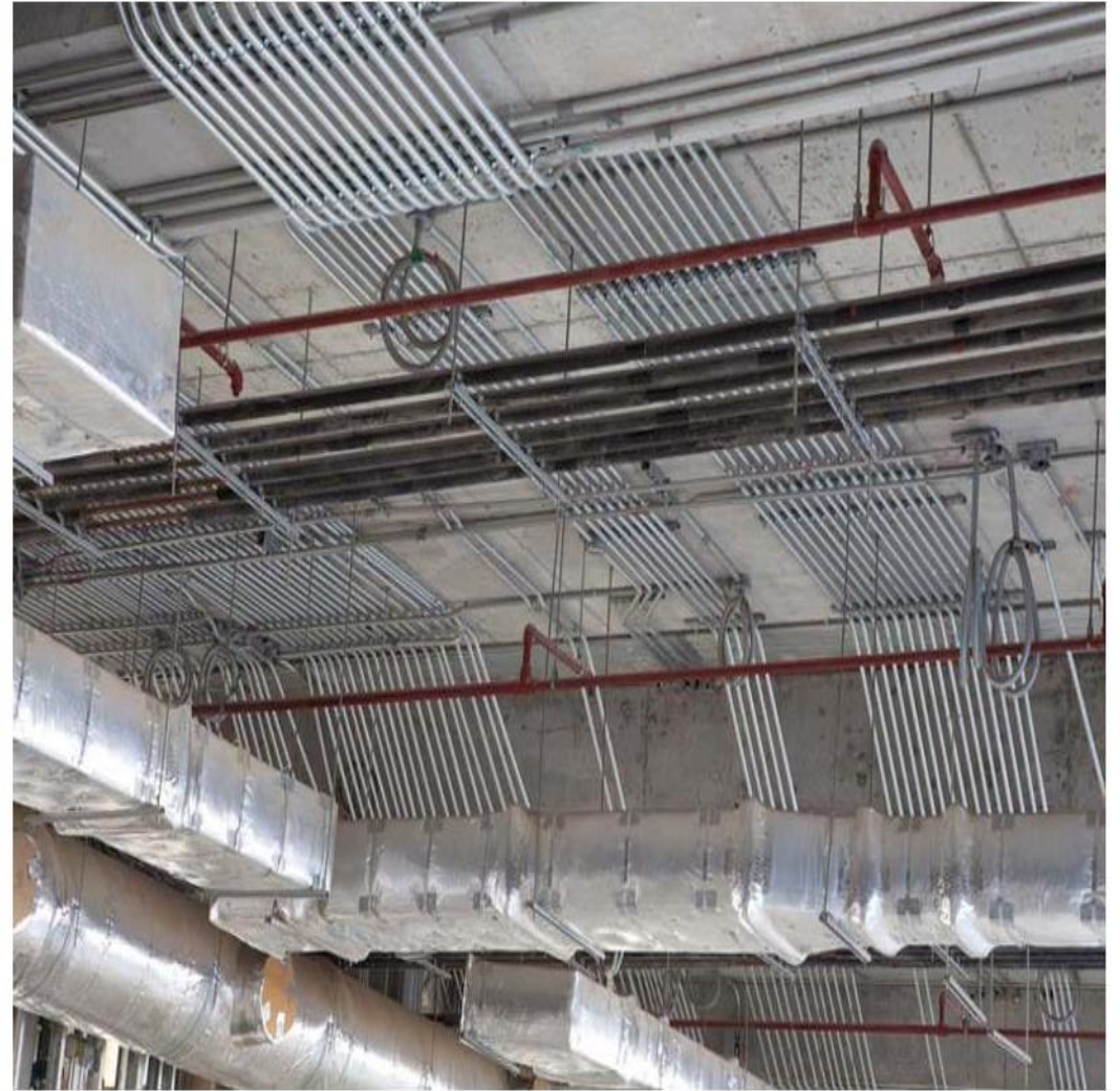
EMT ELECTRICAL SYSTEMS LAY OUT
