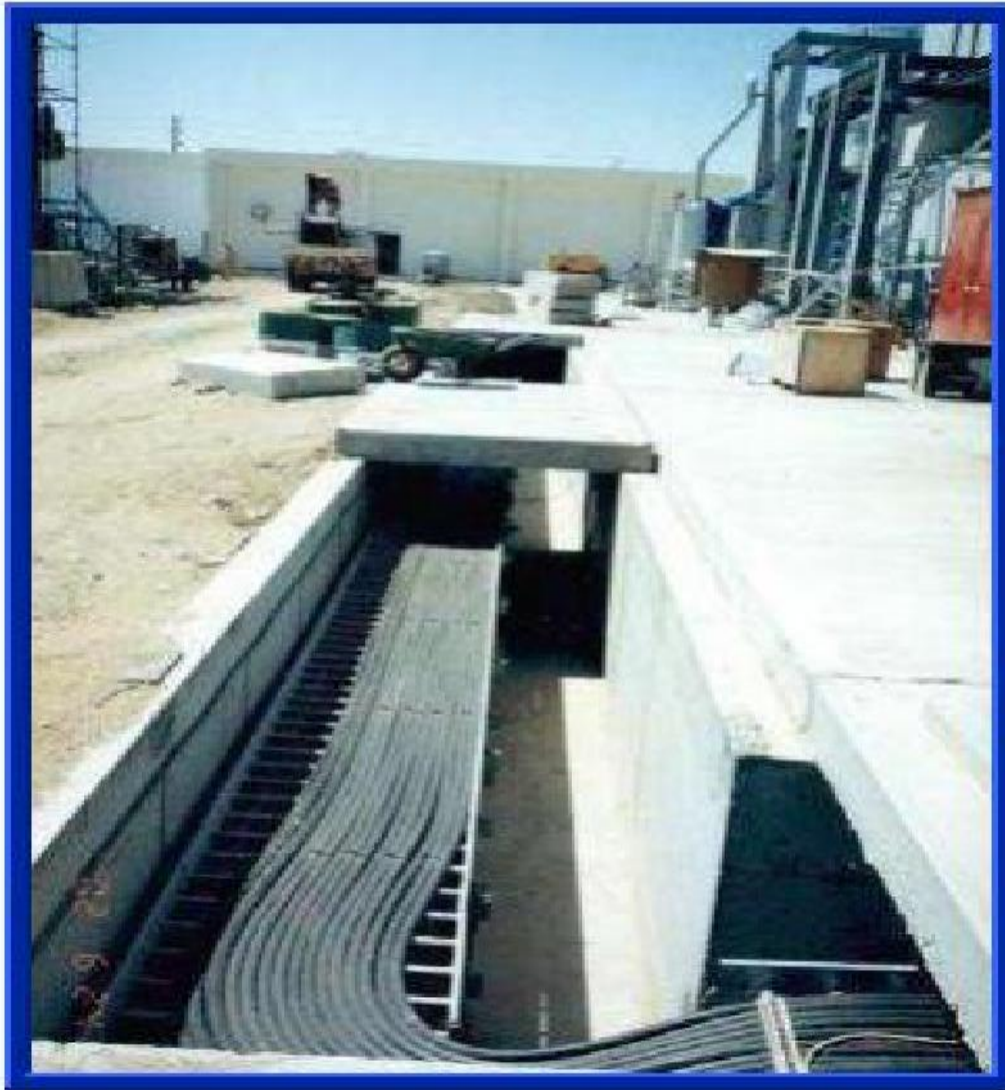
SUB CABLE ELECTRICAL SYSTEMS WORKS
